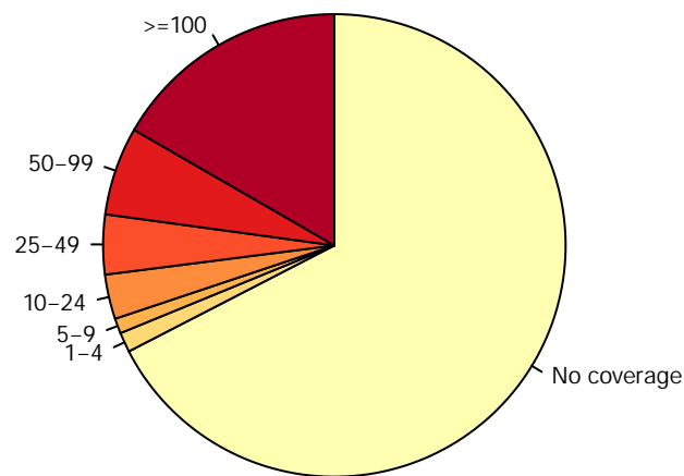
Mouse_blood_erythroblast_S45_rep1.RRBS
