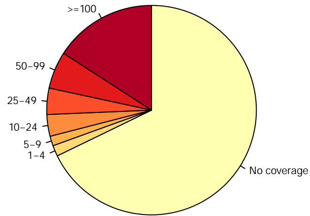
Mouse_blood_erythroblast_S0_rep1.RRBS
