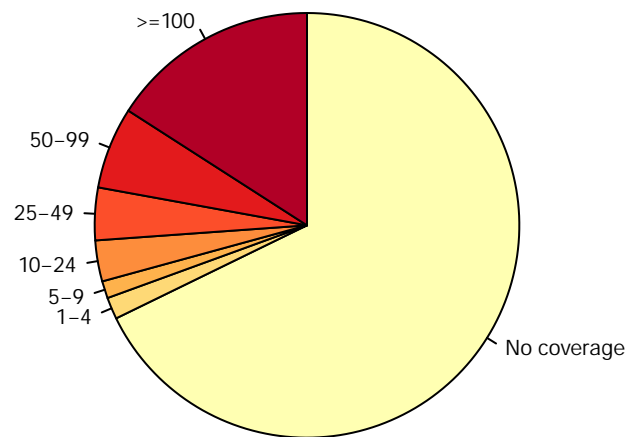
Mouse_blood_erythroblast_S1_rep2.RRBS
