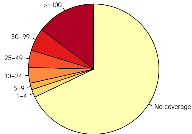
Mouse_blood_erythroblast_S3_rep1.RRBS
