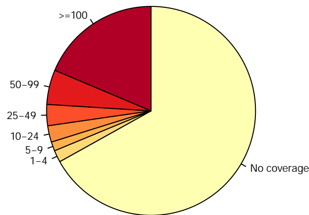
Mouse_blood_erythroblast_S1_aphi_rep2.RRBS
