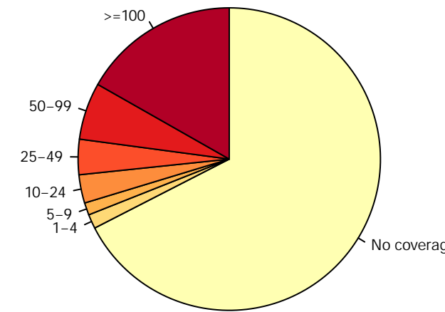
Mouse_blood_erythroblast_S1_rep1.RRBS
