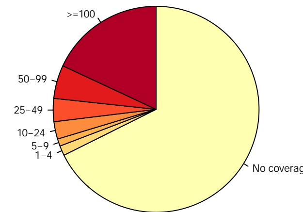
Mouse_blood_erythroblast_S3_rep2.RRBS
