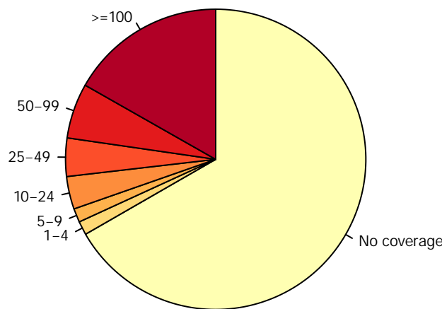
Mouse_blood_erythroblast_S1_ctrl_rep1.RRBS
