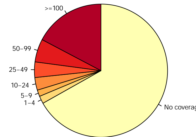
Mouse_blood_erythroblast_S1_aphi_rep1.RRBS
