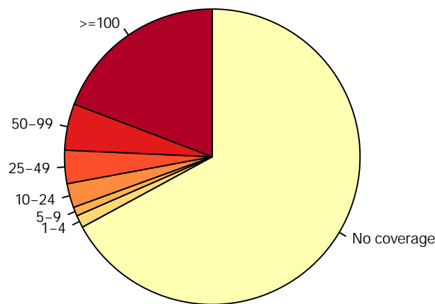
Mouse_blood_erythroblast_S45_rep2.RRBS
