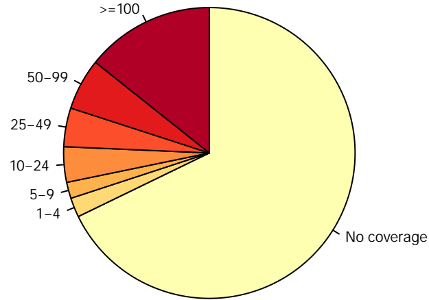
Mouse_blood_erythroblast_S0_rep2.RRBS
