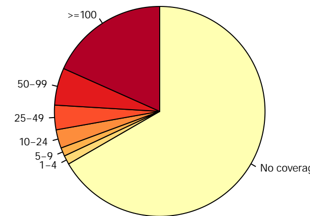
Mouse_blood_erythroblast_S1_ctrl_rep2.RRBS
