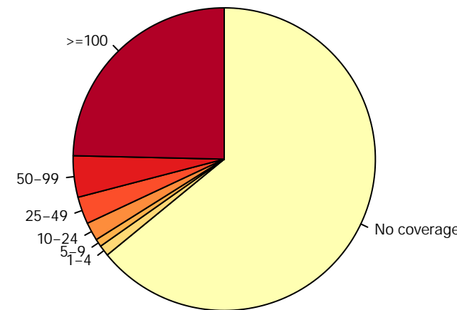
Mouse_blood_erythroblast_S1_rep1.RRBS
