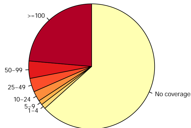
Mouse_blood_erythroblast_S1_ctrl_rep1.RRBS
