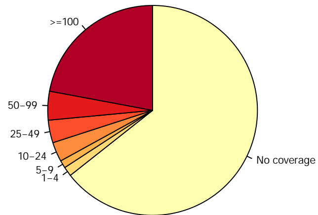
Mouse_blood_erythroblast_S0_rep2.RRBS
