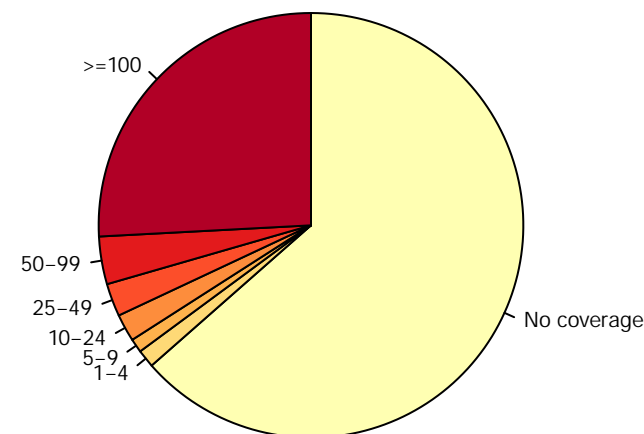
Mouse_blood_erythroblast_S1_aphi_rep2.RRBS
