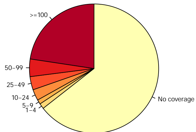
Mouse_blood_erythroblast_S3_rep1.RRBS
