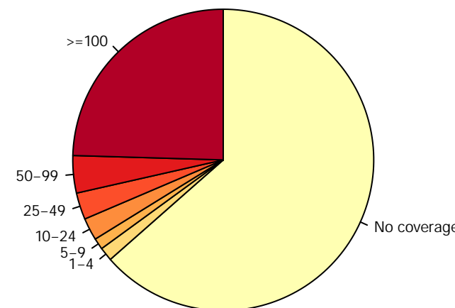
Mouse_blood_erythroblast_S1_aphi_rep1.RRBS
