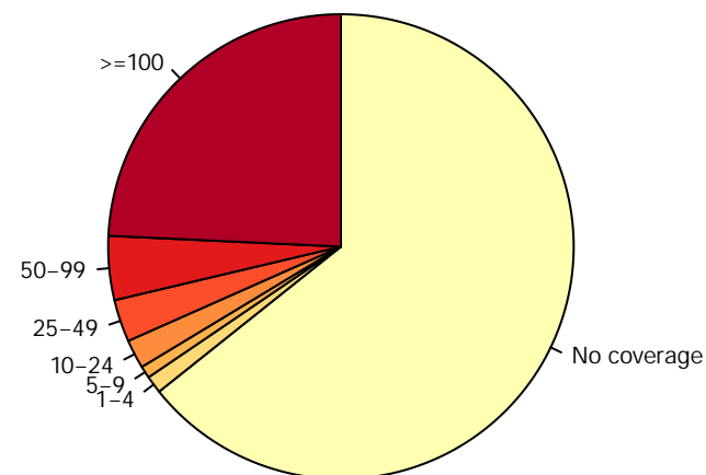
Mouse_blood_erythroblast_S1_rep2.RRBS
