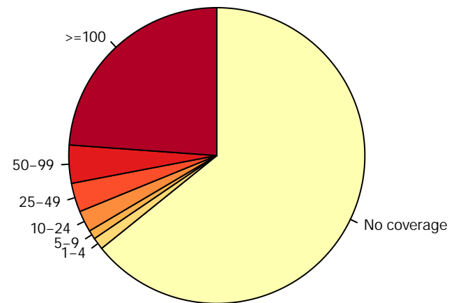
Mouse_blood_erythroblast_S0_rep1.RRBS
