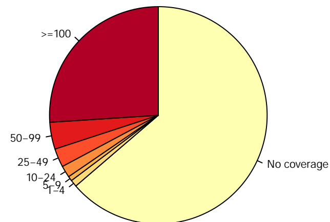
Mouse_blood_erythroblast_S45_rep2.RRBS
