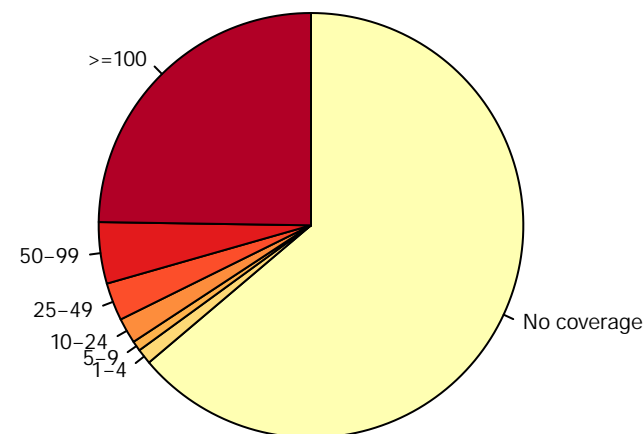
Mouse_blood_erythroblast_S45_rep1.RRBS
