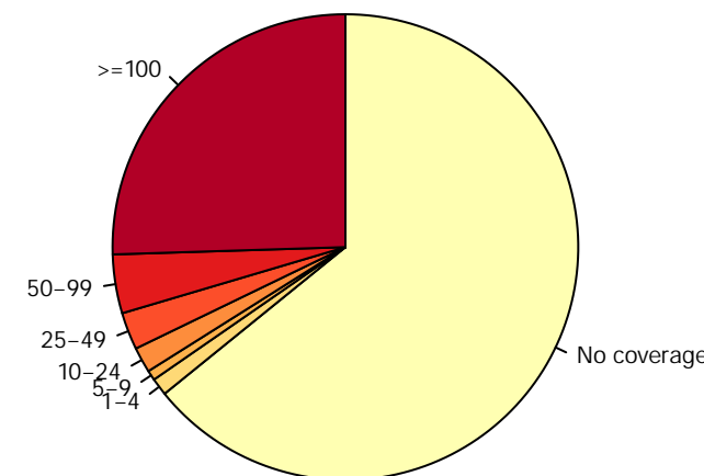
Mouse_blood_erythroblast_S3_rep2.RRBS
