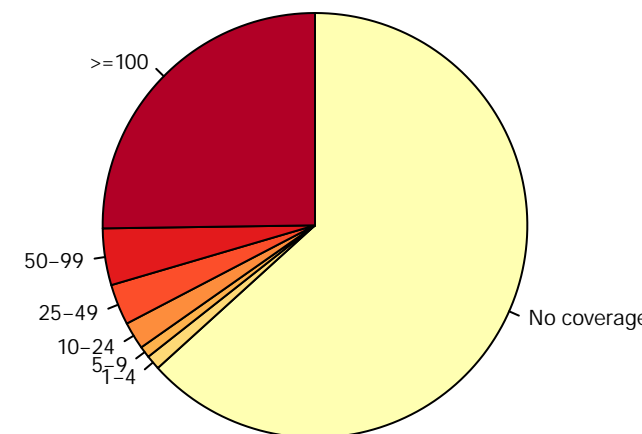
Mouse_blood_erythroblast_S1_ctrl_rep2.RRBS
