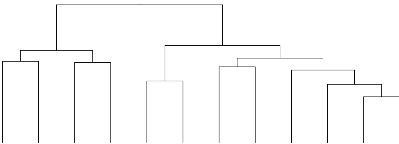
Clustering by samples for: Conserved_Region (yellow: high, red: low)
