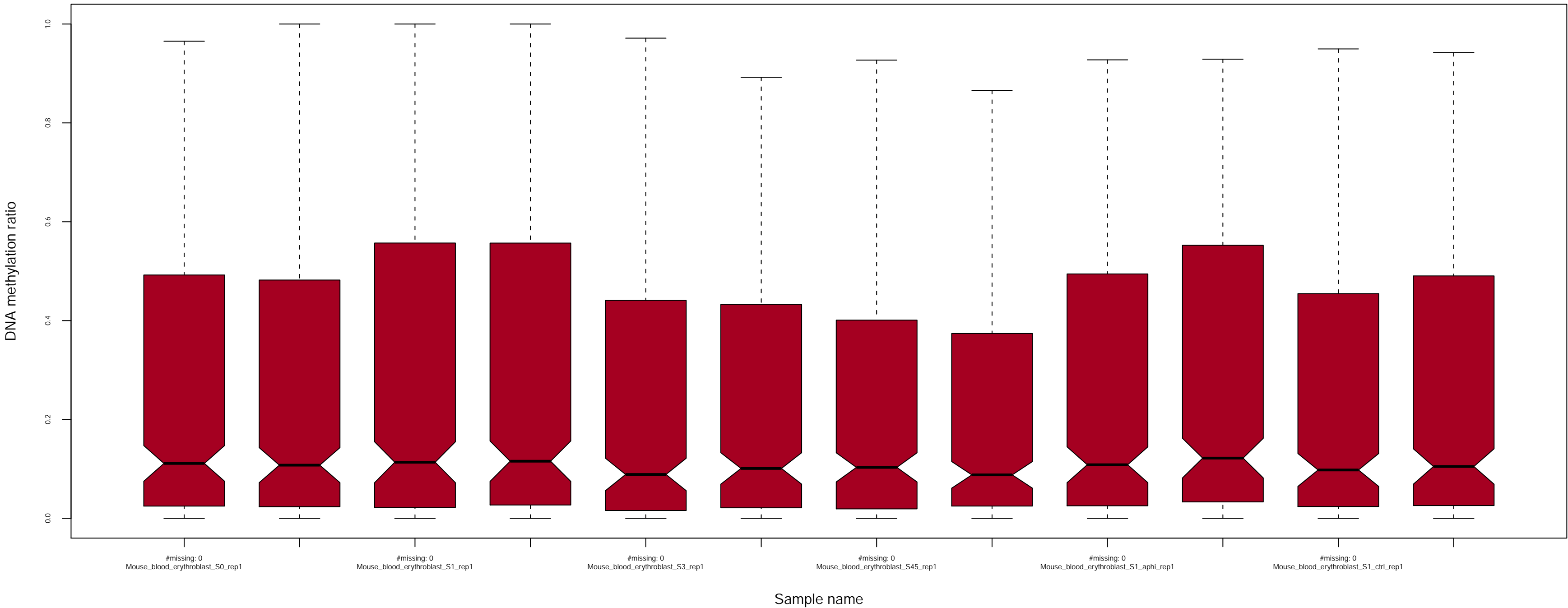
Enhancer_p300 (#regions: 419) – Mean DNA methylation levels
